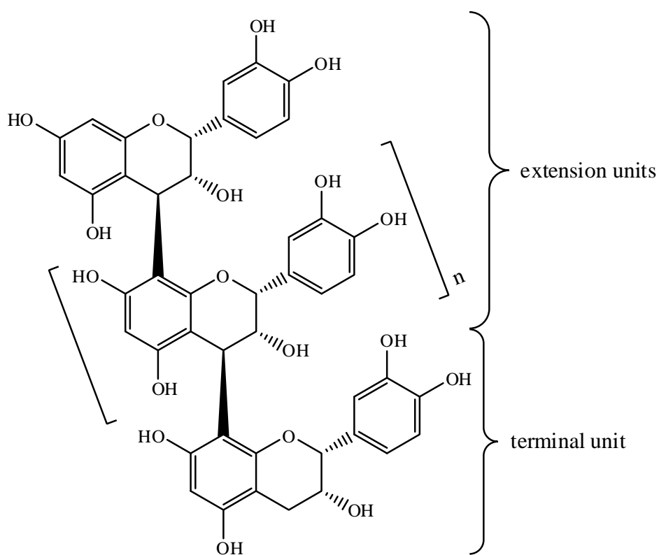
Procyanidin B-type polymer
